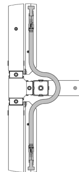
THREE OR FOUR-WAY FRAME SPAN (EDJT)
