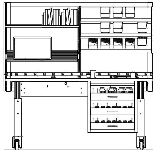
Elevation D
