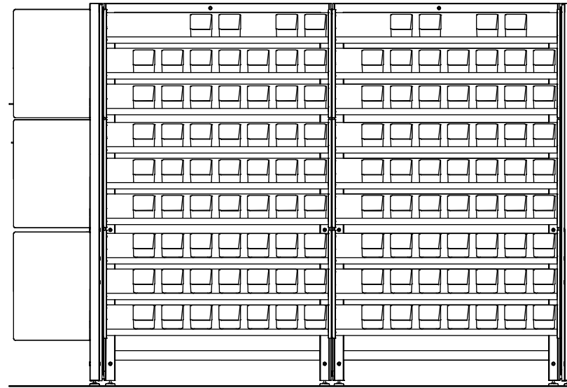
Elevation F
